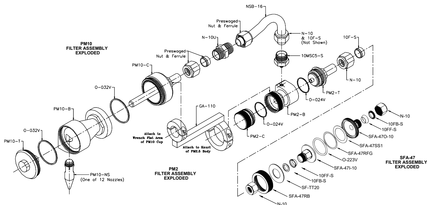
Exploded View of the PM10 and PM2.5 Combination
